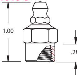
1/8" NPTF FEMALE
